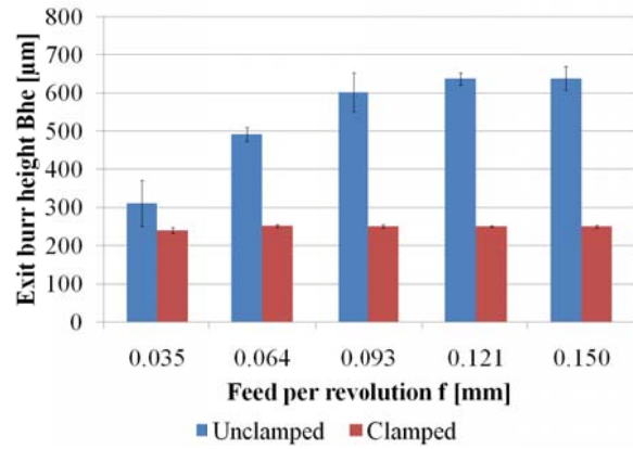
Fig.8. Effect of clamping on exit burr height.
