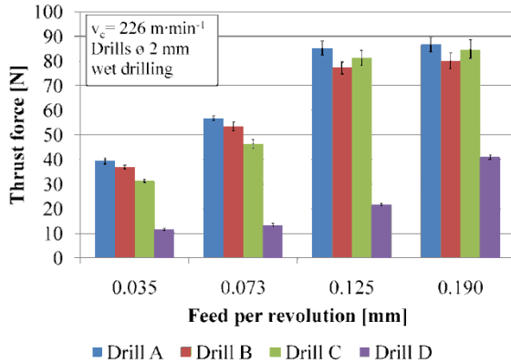
Fig.10. Comparison of drilling thrust force using 4 different drills.
