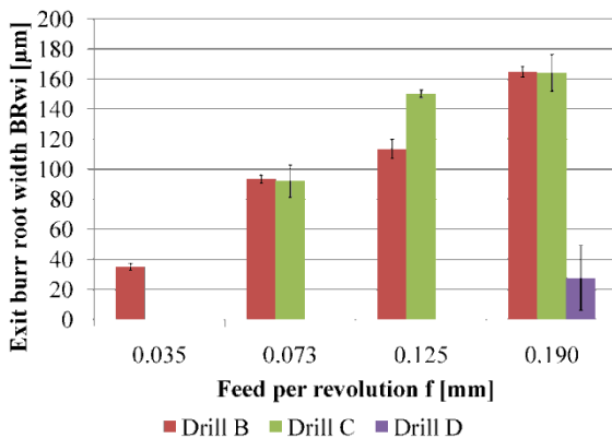
Fig.11. Comparison of exit burr root widths using 3 different drills (Drill A excluded).
