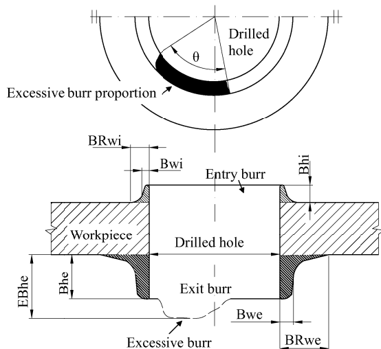
Fig.1. Description of measured burr geometry, where: Bhe – exit burr height, Bhi – entry burr height, BRwe – exit burr root width, BRwi – entry burr root width, Bwe – exit burr width, Bwi – entry burr width, EBhe – Excessive burr height, \theta – angular proportion of excessive burr.
