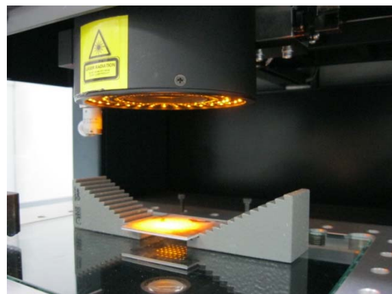
Fig.3. Workpiece fixture when burr widths measured by an optical CMM.
