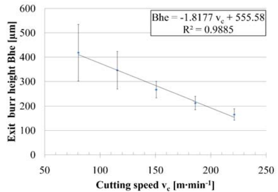
Fig.5. Influence of cutting speed on exit burr height.
