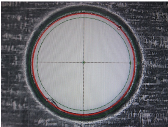
Fig.4. Measuring principle for burr widths based on circle fitting to the burr edges on the CMM.
