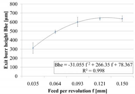
Fig.6. Influence of feed rate on exit burr height.
