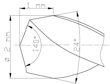
Fig.9. Profile of double cone point drill A.
