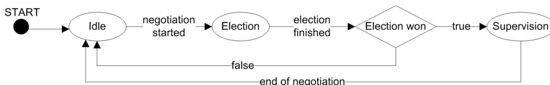
Figure 4. Manager agent state diagram.
