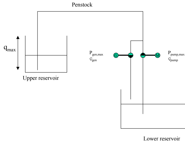
Figure 9 Pumped storage model
