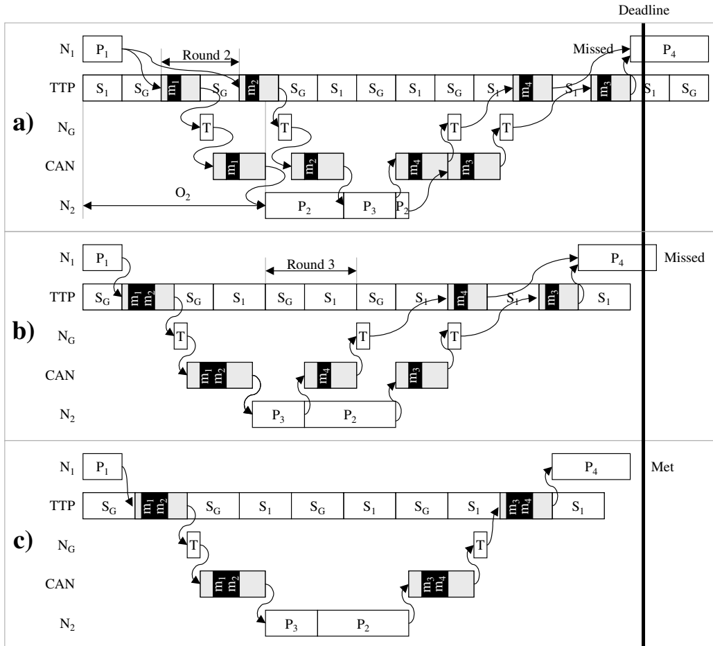
Figure 6. Frame-Packing Optimization Example
