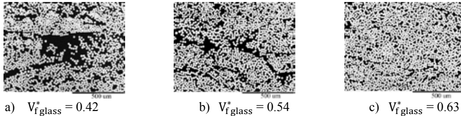
Fig. 5. Examples of determined local glass fibre volume fractions in three areas of a glass fibre composite region.
