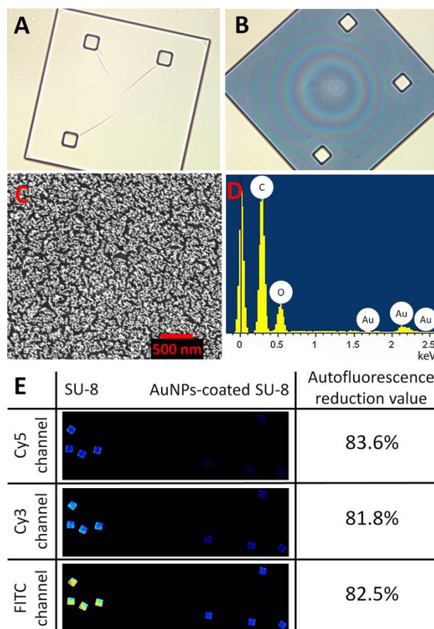
Figure 1. Optical images of a SU-8 microparticle before (A) and after (B) deposition of the AuNPs (at 200\times magnification). (C) Surface characterization of a Au-coated SU-8 microparticle by scanning electron microscopy (SEM) and (D) energy-dispersive spectroscopy (EDS-SEM) demonstrating the Au layer deposited on the SU-8 surface. (E) shows reduction in autofluorescence of the Au-coated SU-8 surface for the different wavelength ranges: Cy3, Cy5 and FITC.
