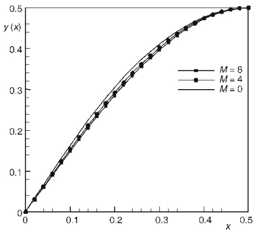
Figure 1. Variation of y(x) for different values of M for \alpha = 0.2, \text{Re} = 2 : (HAM and VIM)
