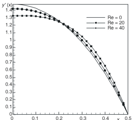
Figure 3. Variation of dy(x)/dx for different values of \text{Re} for \alpha = 0.2, M = 2 : (HAM and VIM)
