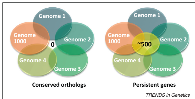
Figure 1. Different criteria for defining universally conserved genes. When 1000 genomes are compared via comparative genomics, the number of orthologous genes falls to 0 (left), but this number can increase to about 500 persistent genes by comparing orthologs that belong to a quorum of a similar or different genomes from evolutionarily distinct bacteria, above a threshold computed using a measure that retains frequent genes that tend to cluster together (right).
