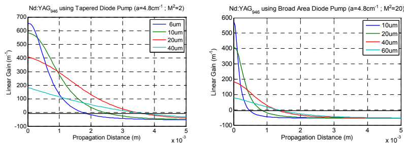
Fig. 1 Numerical calculation of non-saturated gain at 946 nm in Nd:YAG for tapered diode pump (left) and broad-area diode pump (right.)
