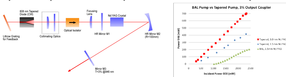
Fig. 2 Experimental setup (left) and results (right) of a 946 nm Nd:YAG laser pumped by a tapered diode laser and broad-area diode laser.
