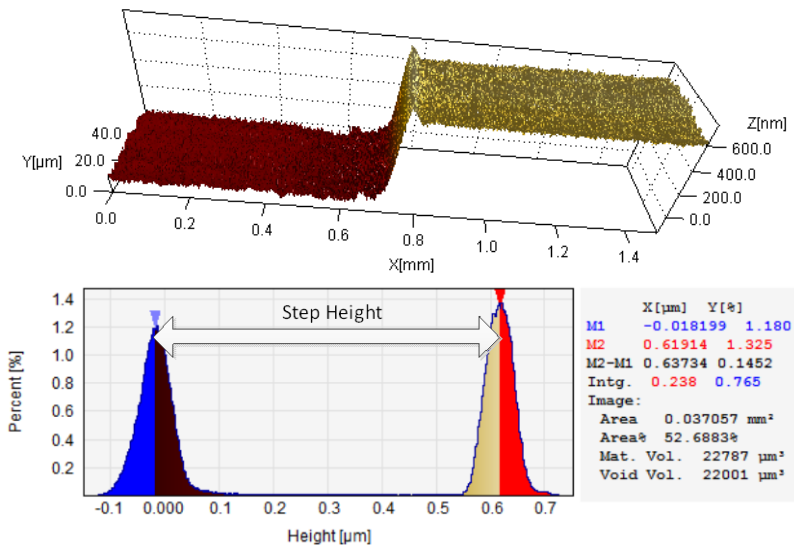
Figure 1: Height measurement of HSQ layer by 3D stylus including the height histogram
