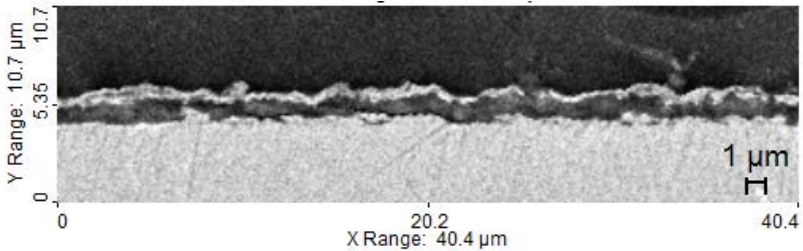
Figure 2: SEM image of the substrate (bottom) coated with HSQ (middle black layer) and an additional Ni layer (white thin layer in the middle of the picture)
