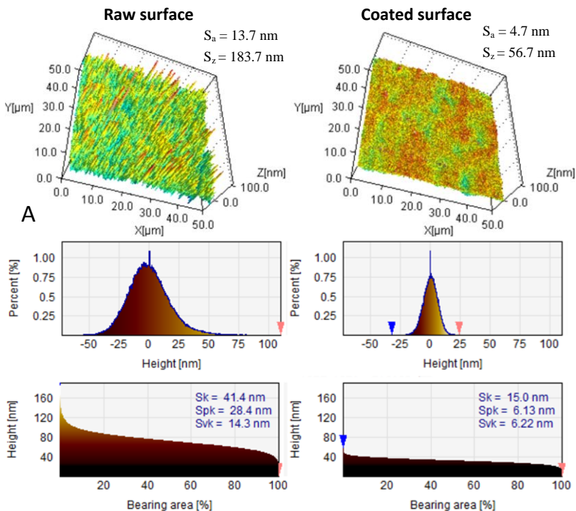
Figure 3: 3D surface characterisation of raw (left) and HSQ coated surface (right): visualisation (A), height histogram (B) and bearing curves (C)
