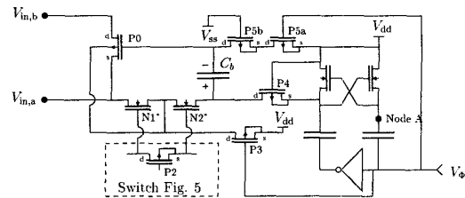
Figure 7: Low-voltage low-stress (gate oxide) implementation.
