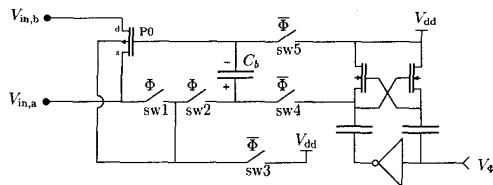
Figure 6: Body-effect-compensated bootstrapped switch.
