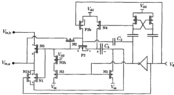
Figure 5: Bootstrapped switch.
