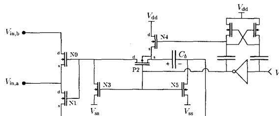
Figure 4: Bootstrapped switch: simple implementation.
