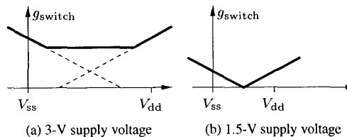
Figure 2: On-state conductance of the transmission-gate switch.
