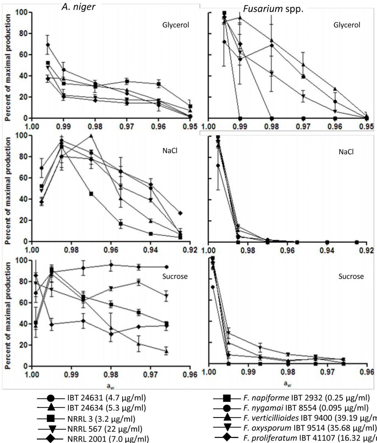
Figure 2 Effect of glycerol, NaCl and sucrose on the FB 2 production of Aspergillus niger and the total production of FB 1 , FB 2 and FB 3 by F. verticillioides , F. proliferatum , F. napiforme , F. nygamai and F. oxysporum . Strains have been incubated at 25°C for 7 days on CYA or PDA. The concentration of fumonisins were detected in the methanol:water (3:1) extract. The values are means of biological duplicates on two different plates, highest value is in parenthesis.
