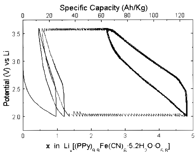
Figure 5. Discharge and charge cycles of a lithium cell where the positive electrode is a thin film made from PPy/HCF (obtained at 0°C) using PVDF and carbon Super P. V_{\text{initial}} = 2.97 V, V_{\text{min}} = 2.0 V, V_{\text{max}} = 3.6 V, I_{\text{discharge}} = I_{\text{charge}} = 25 \mu\text{A} . Only cycles 1, 2, and 55-60 are shown for clarity.
