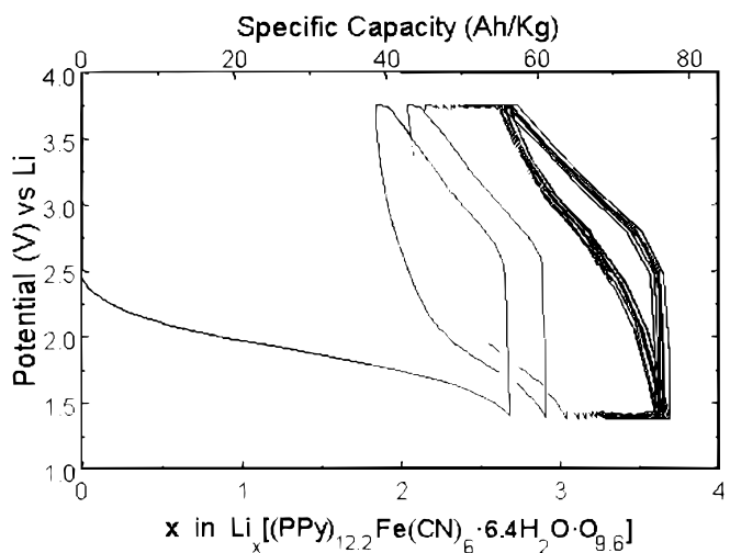
Figure 7. First discharge and charge cycles of a lithium cell where the positive electrode is a thin film made from PPy/HCF (obtained at 42°C) using PVDF and carbon Super P. V_{\text{initial}} = 2.45 V, V_{\text{min}} = 1.4 V, V_{\text{max}} = 3.75 V, I_{\text{discharge}} = I_{\text{charge}} = 100 \mu\text{A} . Only cycles 1, 2, and 55-60 are shown for clarity.
