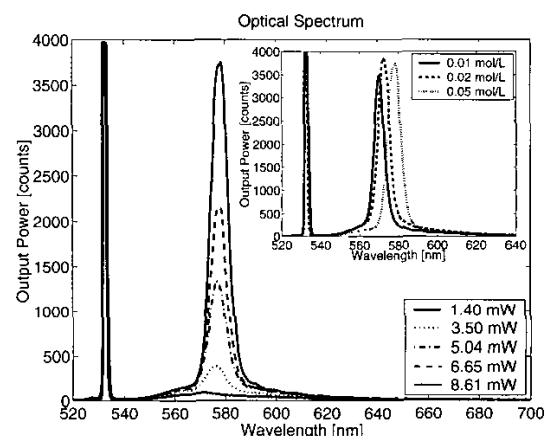
Figure 6: Measured spectra emitted from the micro-cavity fluidic dye laser, using a dye solution of 5 \cdot 10^{-2} mol/L Rhodamine 6G in ethanol and a flow rate of 10 \mu\text{L}/\text{min} . The spectra are recorded with different levels of optical pumping power (average power). The first peak at 532 nm is due to scattered pump laser light. A strong peak from the dye laser appears at around a wavelength of 578 nm. The insert shows three dye laser spectra for three dye concentrations 10^{-2} , 2 \cdot 10^{-2} , and 5 \cdot 10^{-2} mol/L. The lasing peak wavelength is shifted towards longer wavelength for increasing dye concentration. The peak wavelength for the three spectra are: 570 nm, 572 nm, and 578 nm, respectively.
