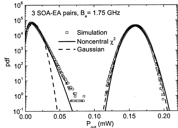
Fig. 10. Noise distribution after three SOA-EA pairs for a bandwidth of 1.75 GHz.
