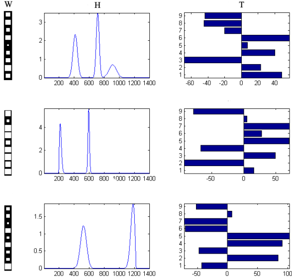
Fig. 2. The true factors forming a synthetic data set. To the left, the strength of the mixing W of each source is indicated in gray color scale. In the middle, the three sources are shown and to the right is given the time delays of each source to each channel.
