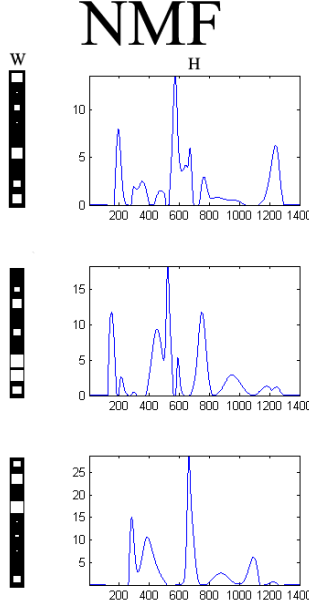
Fig. 4. Results obtained by regular instantaneous NMF for the synthetic data given in gure 3. To the left, the strength of the mixing W of each source is indicated in gray color scale. In the middle, the three sources are shown. Clearly, since the model can't account for the shifts in the data the sources estimated are mixtures of the 3 true sources. Notice, only 68 % of the variance of the data is accounted for.
