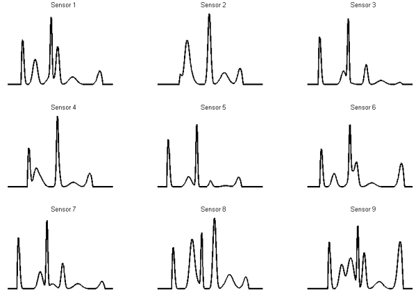
Fig. 3. The synthetic dataset generated from the factors given in gure 2 when mixed into each of the 9 sensors.
