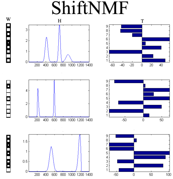
Fig. 5. The estimated factors obtained by a ShiftNMF analysis of the synthetic data given in gure 3. To the left, the strength of the mixing W of each source. In the middle, the three sources are shown and to the right is given the time delays of each source to each channel. Clearly, the model with shifts has correctly recovered the components of the synthetic data hence accounts for all the variance in the data.
