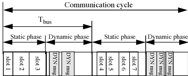
Fig. 5. Mixed communication cycle.
