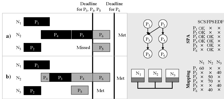
Fig. 14. Scheduling policy assignment example #1.
