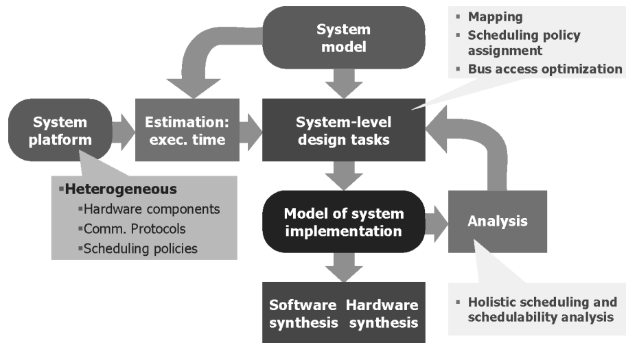
Fig. 9. System-Level design flow example.
