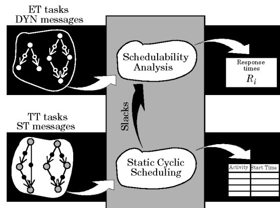
(a) TT and ET resource sharing
