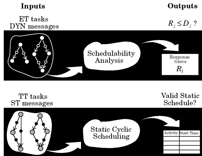
Fig. 10. Timing analysis for isolated TT and ET domains.
