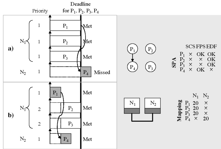
Fig. 15. Scheduling policy assignment example #2.
