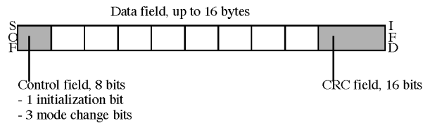
Fig. 2. Time-Triggered Protocol.
