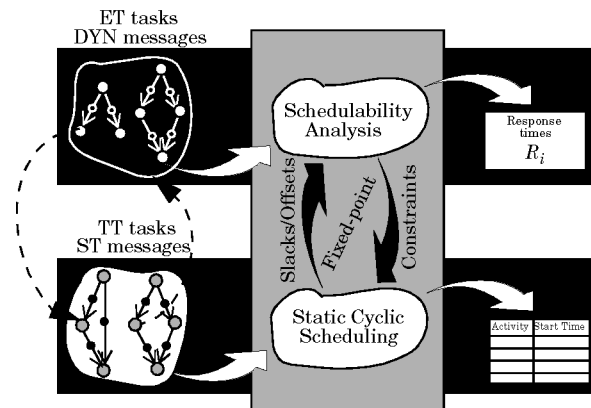
(b) TT and ET resource sharing and communication
