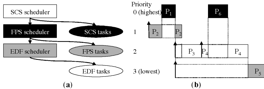
Fig. 6. Heterogeneous scheduling policies.
