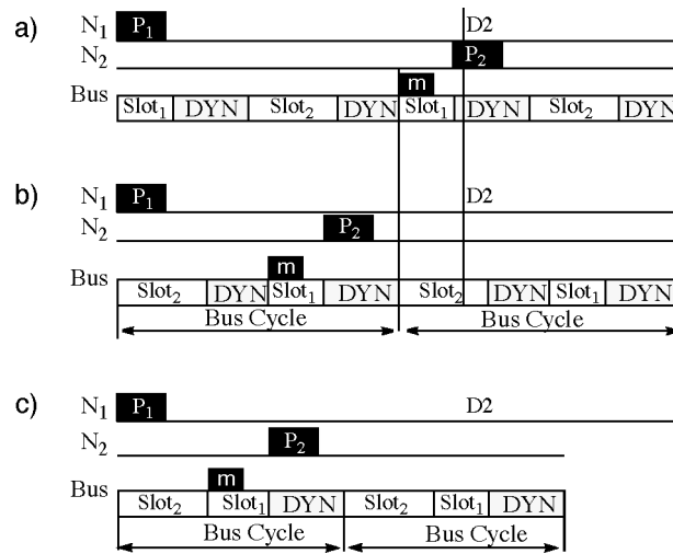
Fig. 13. Optimization of bus access cycle.
