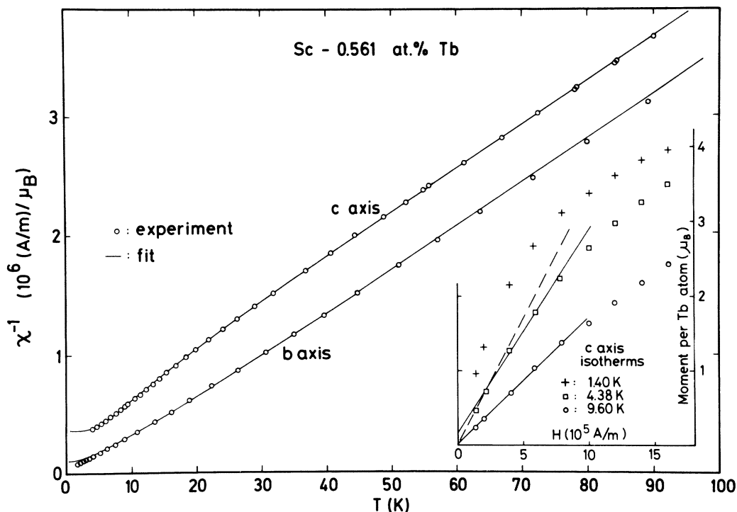
FIG. 1. Reciprocal susceptibility for Sc-0.561-at.% Tb. The full curves are theoretical fits. The susceptibility measured as the ratio \chi_H = M/H at H = 1.35 \times 10^5 \text{ A/m} has been corrected in the c direction below 9 K to the differential susceptibility \chi_{CF} obtained from isothermal magnetization curves as illustrated in the inset. The dashed line and the upper full line have the slopes \chi_H (4.38 K) and \chi_{CF} (4.38 K), respectively. The lower full line has the slope \chi_H (9.60 K) = \chi_{CF} (9.60 K). At 4 K the accuracy of \chi_{CF} is \pm 7\% . Below 4 K \chi_{CF} cannot be obtained with reasonably accuracy.
