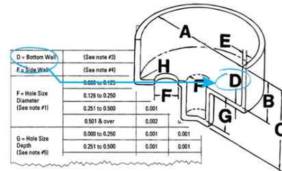
Fig. 3. Available tolerance guidelines for injection moulding processes (picture adopted from [11])
