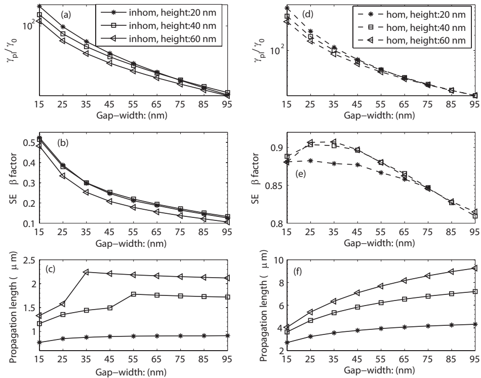
Fig. 4. Gap-width dependence of the plasmonic decay rates, SE \beta -factors, and the propagation length of the gap mode for an inhomogeneous dielectric environment (a, b, c) and for a homogenous dielectric environment (d, e, f). In the subplot (a, b, c), n_c = 1.5 , W = 100 nm and n_s = 3.5 , while for homogenous case in the subplot (d, e, f), the surrounding material is air ( n_{air} = 1.0 ), and W = 100 nm.
