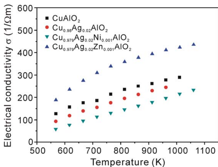
Figure 3. Temperature dependence of the electrical conductivity \sigma of \text{CuAlO}_2 , \text{Cu}_{0.98}\text{Ag}_{0.02}\text{AlO}_2 , \text{Cu}_{0.979}\text{Ag}_{0.02}\text{Ni}_{0.001}\text{AlO}_2 and \text{Cu}_{0.979}\text{Ag}_{0.02}\text{Zn}_{0.001}\text{AlO}_2 samples.
