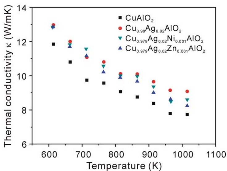
Figure 6. Temperature dependence of the thermal conductivity \kappa for the samples.
