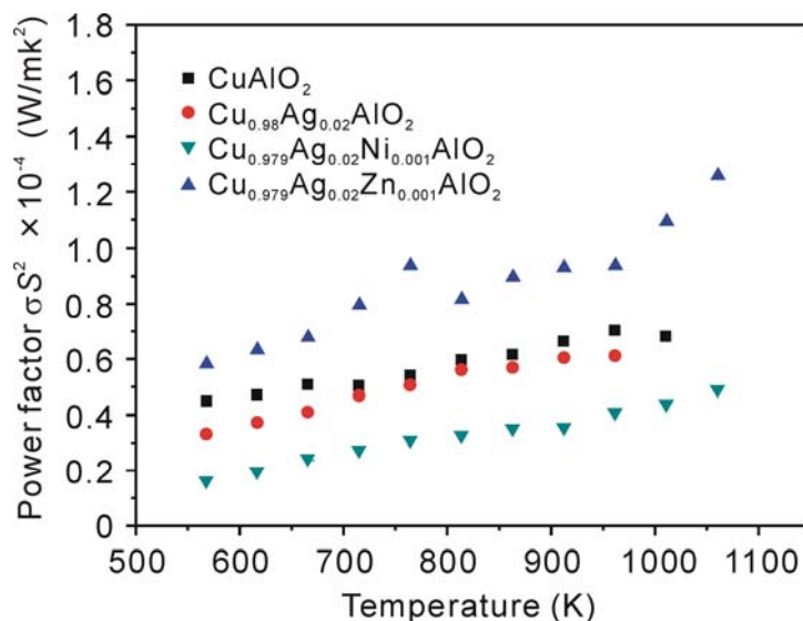
Figure 5. Temperature dependence of the power factor of \text{CuAlO}_2 , \text{Cu}_{0.98}\text{Ag}_{0.02}\text{AlO}_2 , \text{Cu}_{0.979}\text{Ag}_{0.02}\text{Ni}_{0.001}\text{AlO}_2 and \text{Cu}_{0.979}\text{Ag}_{0.02}\text{Zn}_{0.001}\text{AlO}_2 samples.
