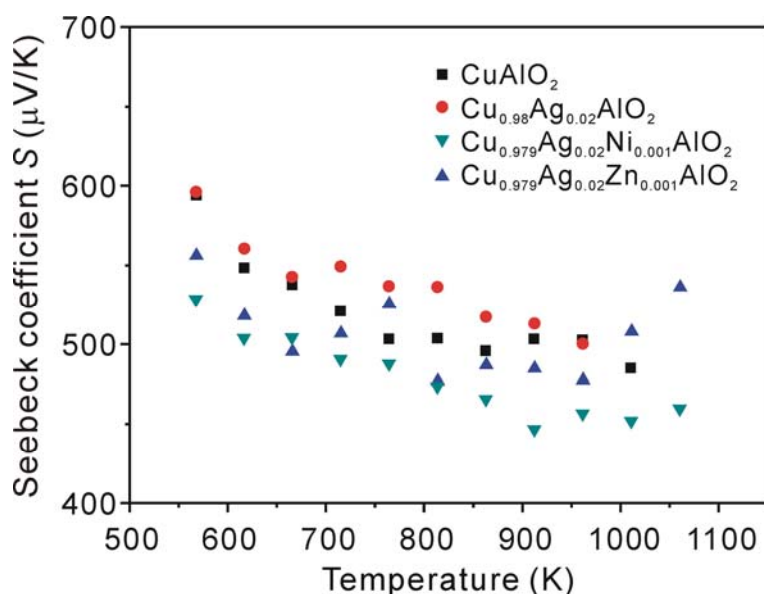
Figure 4. Temperature dependence of the Seebeck coefficient S of CuAlO 2 , Cu 0.98 Ag 0.02 AlO 2 , Cu 0.979 Ag 0.02 Ni 0.001 AlO 2 and Cu 0.979 Ag 0.02 Zn 0.001 AlO 2 samples.
