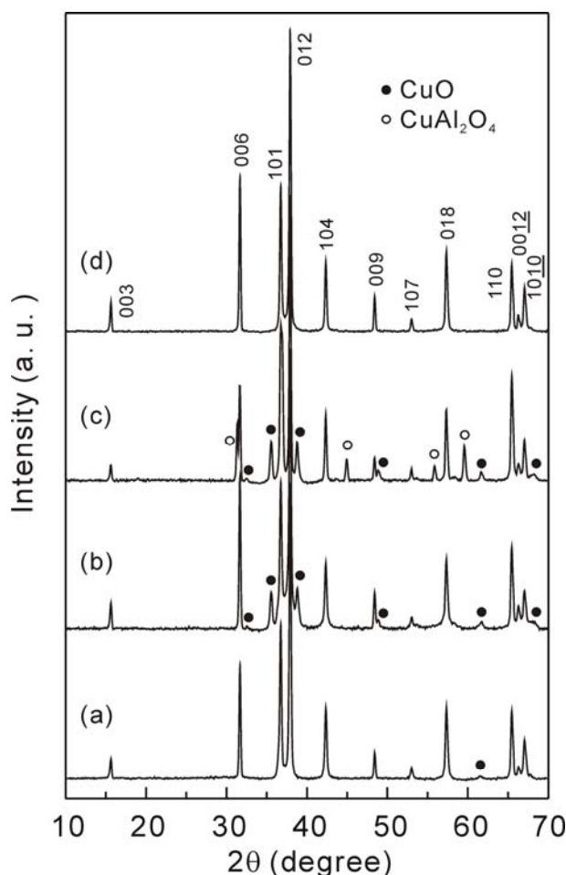
Figure 1. Powder XRD patterns of the samples: (a) \text{CuAlO}_2 , (b) \text{Cu}_{0.98}\text{Ag}_{0.02}\text{AlO}_2 , (c) \text{Cu}_{0.979}\text{Ag}_{0.02}\text{Ni}_{0.001}\text{AlO}_2 and (d) \text{Cu}_{0.979}\text{Ag}_{0.02}\text{Zn}_{0.001}\text{AlO}_2 samples.
