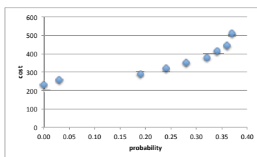
Fig. 3. Pareto optimal solutions.
