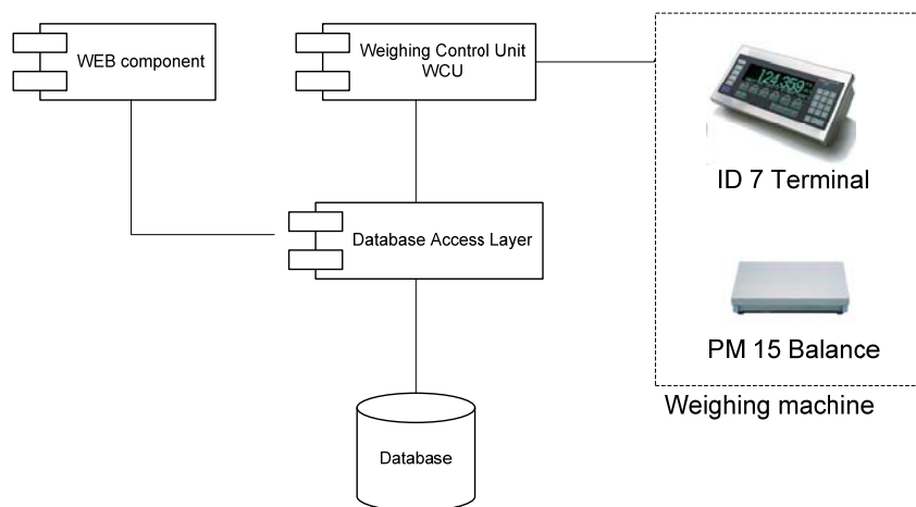
Figure 3: Software architecture
