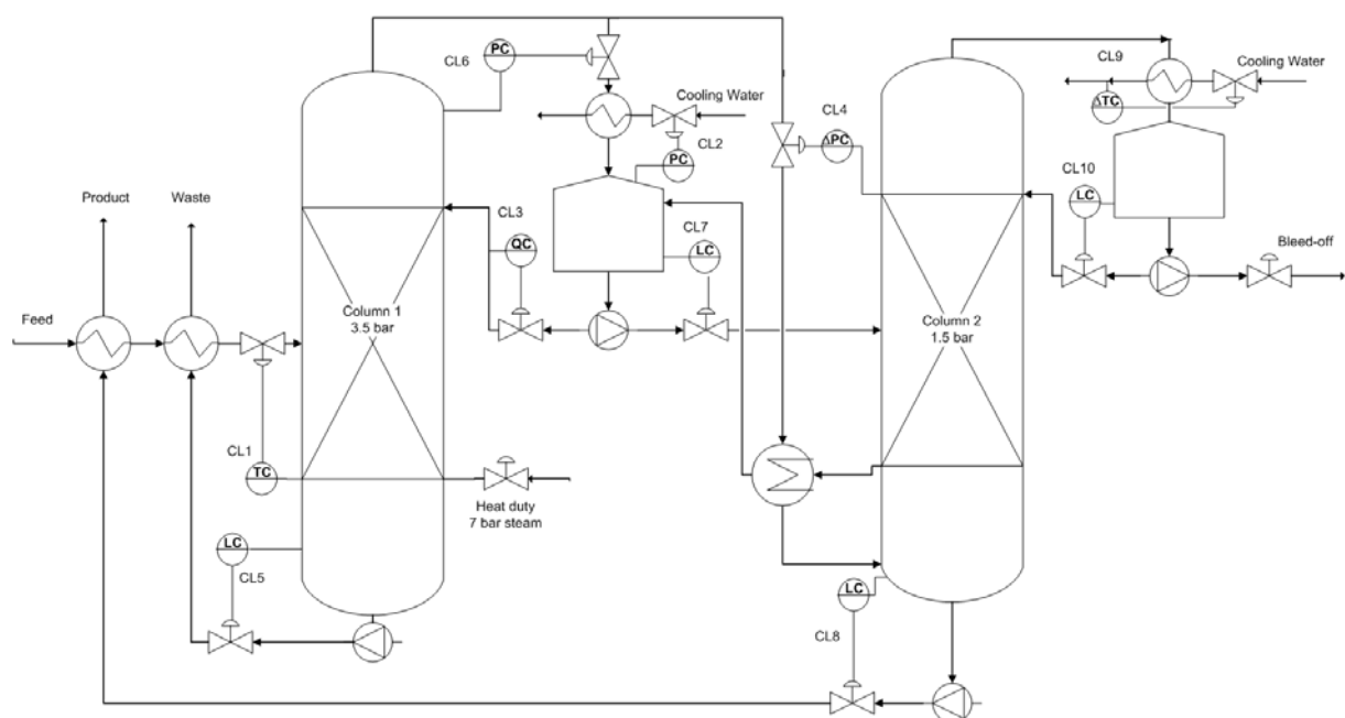
Figure 1. Flowsheet of the plant of ethanol recovery indicating the existing control system
