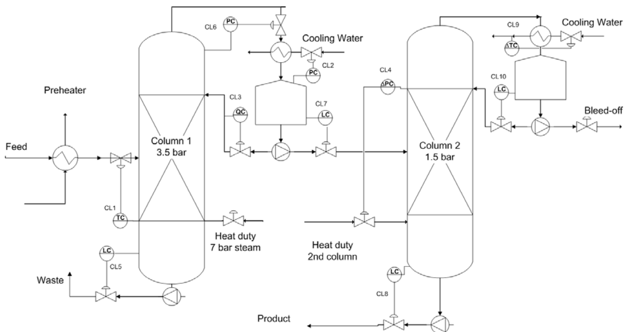
Figure 2. Flowsheet of the alternative plant without heat integration streams
