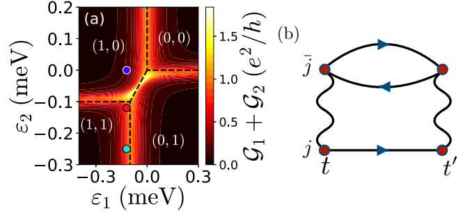
FIG. 2. (a) Stability diagram showing the energetically most favorable dot occupations ( n_1, n_2 ) vs level positions (gate voltage). The honeycomb vertex (dashed lines) connecting the two triple points at the center of the diagram is due to the interdot Coulomb interaction U . The color scale shows the sum of the linear conductances \mathcal{G}_1 + \mathcal{G}_2 in the drive and drag systems. The dots mark the level configurations considered in Fig. 3. Parameters: U = 0.1 meV, \gamma_{L1} = \gamma_{R1} = 7 \mu\text{eV} , \gamma_{L2} = \gamma_{R2} = 25 \mu\text{eV} , D_{\alpha j} = 10 meV, lead coupling shifts \tilde{\varepsilon}_{L1} = -\tilde{\varepsilon}_{R1} = -2.5 meV, and T = 23 mK. (b) Feynman diagram for the single-bubble approximation to the xc part of interaction self-energy in Eq. (3).
