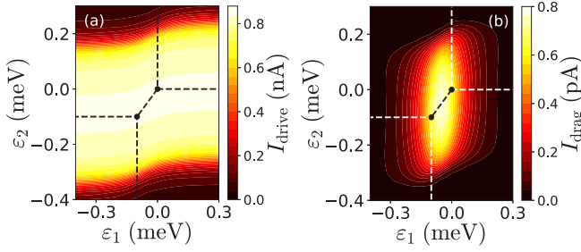
FIG. 4. (a) Drive current and (b) drag current as a function of the level positions \varepsilon_1 and \varepsilon_2 for an applied bias of V = 0.5 mV. All other parameters are the same as in Fig. 2.
