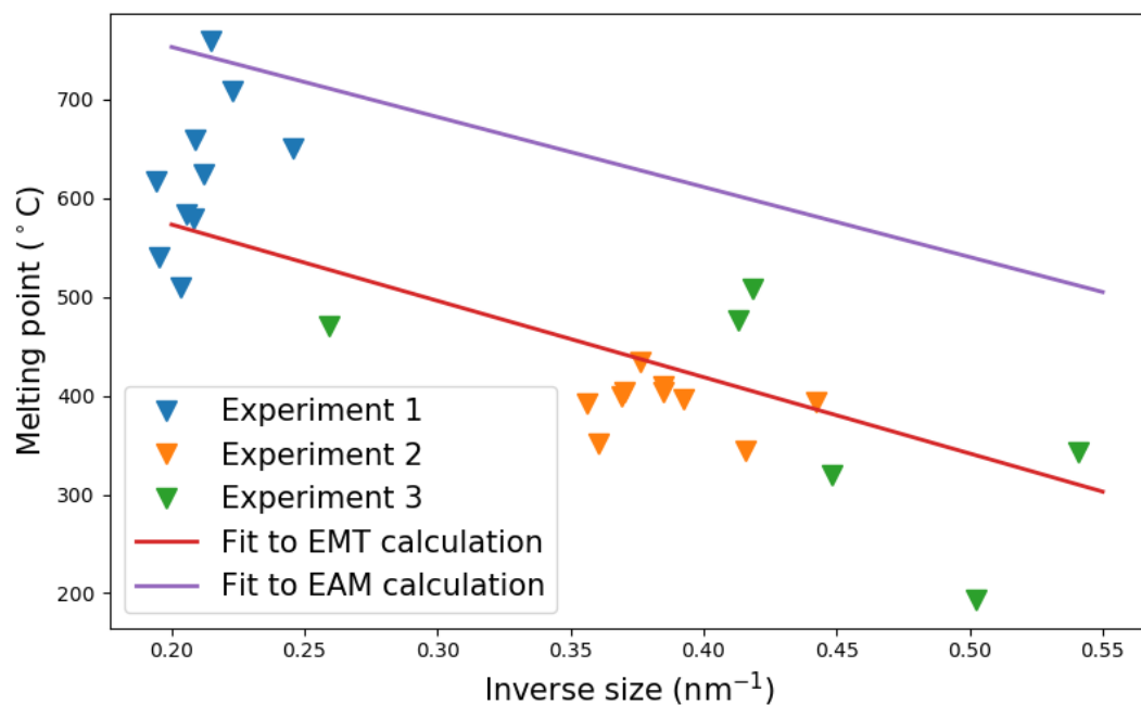
Figure 1: Observed and calculated melting point as a function of inverse particle diameter.
