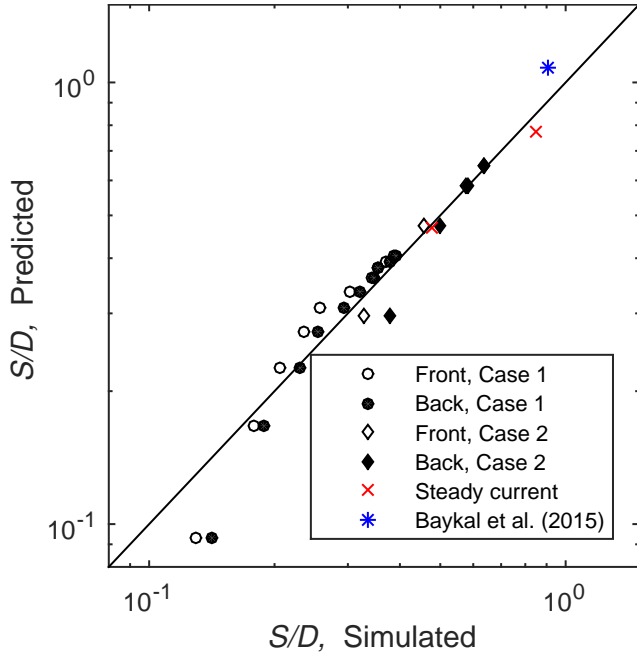
Figure 16: Comparison between the predicted and simulated scour depths.
