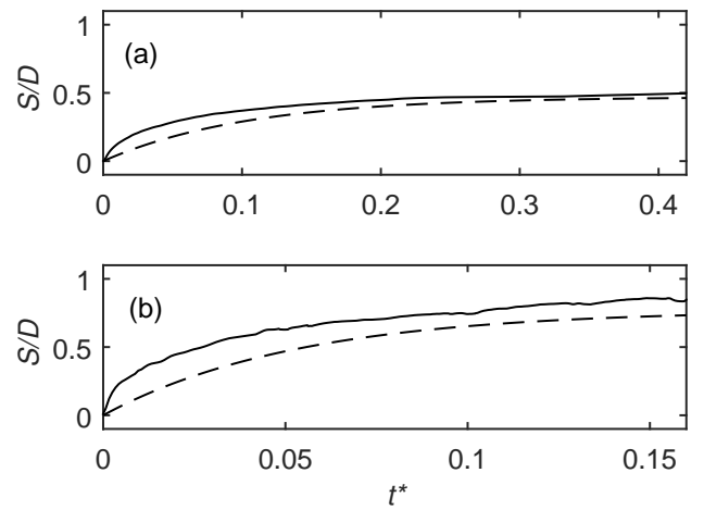
Figure 4: Computed temporal evolution of the scour depth under steady current conditions (full lines) of a) Test 1 and b) Test 2. Also shown (dashed lines) is that from (30) after invoking (24) and (26).
