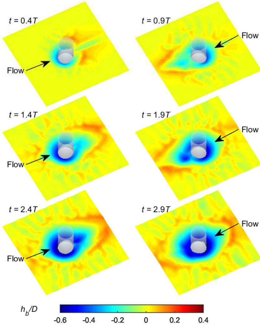
Figure 11: Bed profiles around the monopile for Case 2 for three different periods.
