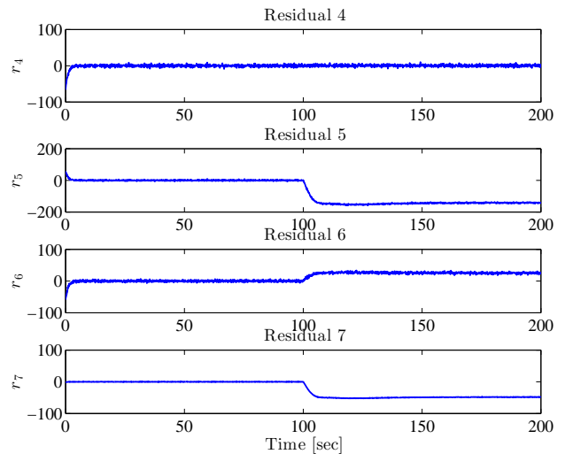
Fig. 5. Residuals during thruster degradation. Fault occurs at time t = 100s .
