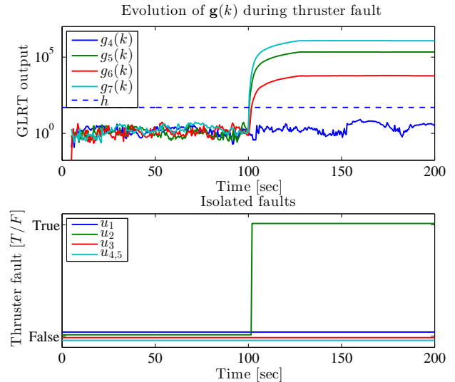
Fig. 4. GLRT output during thruster failure. Fault occurs at time t = 100s . The fault is correctly isolated as u_2 .
