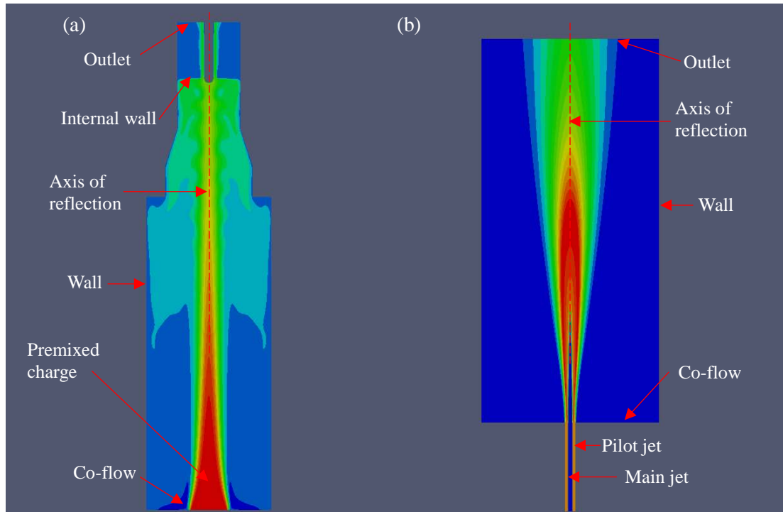
Figure 1. Reflected of the 2-D computational domains of the combustion chambers used for (a) DTU Helium-stabilized laminar premixed flame simulation and (b) Sandia Flame D simulation.
