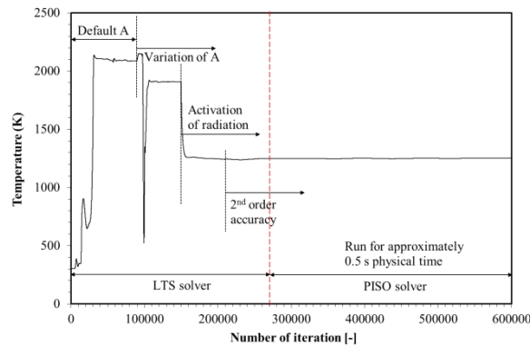
Figure 2. Plot of the convergence criterion of the simulation, the temperature at the height of 150 mm above the burner surface.
