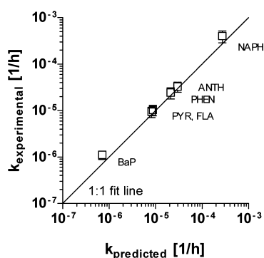
Figure 3. Predicted versus experimental velocity rate constants k for the diffusive mass transfer of PAHs through water with the mean and the standard error of the mean ( n = 3 ) indicated.
