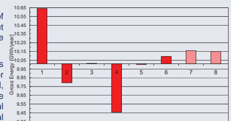
Gross Energy (P50) at hub height. Including results from virtual data, cases 7 and 8. Mean value \pm 6.5\%
