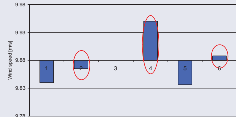
Mean wind speed after filtering at 100 m obtained as mean of ten minutes value. Mean value \pm 1.0\% . Red circles indicates that mast shadow effect has been filtered
