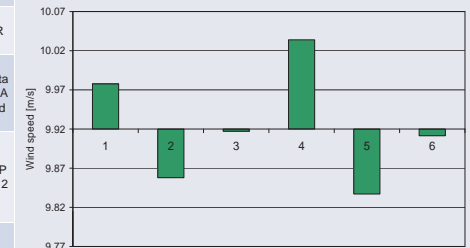
Long term mean wind speed at 100 m obtained from frequency distribution of hours in the year as a function of wind speed and direction. Mean value \pm 1.5\%
