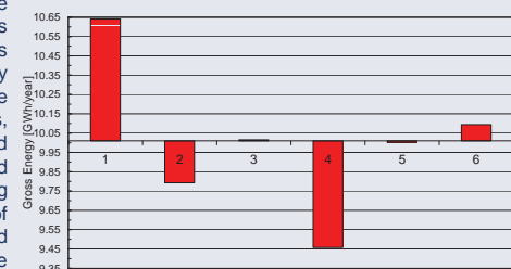
Gross Energy (P50) at hub height. Mean value \pm 6.5\%
