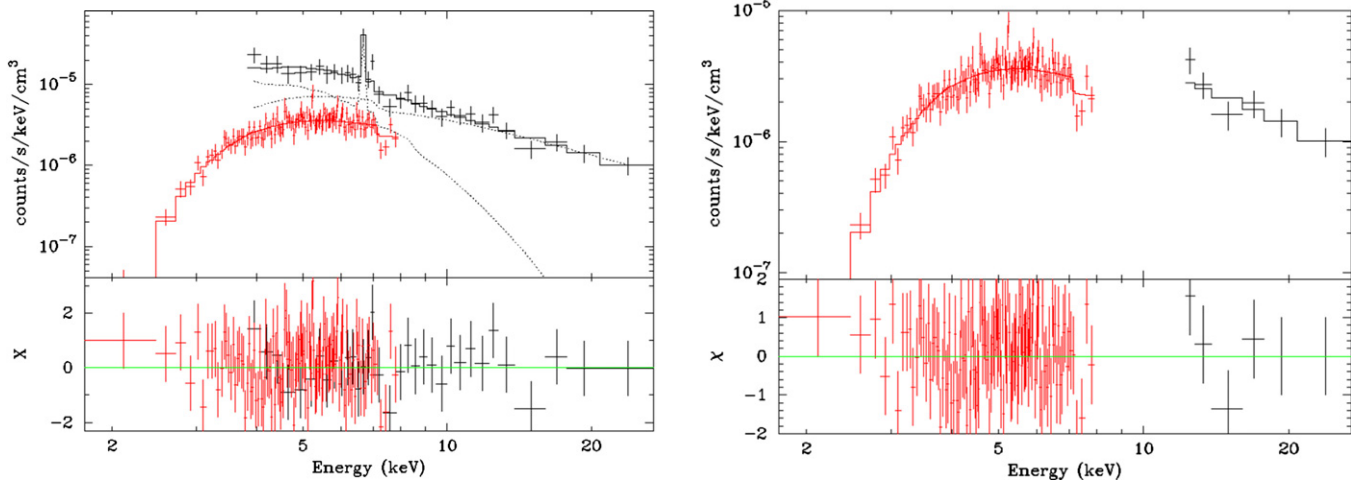
Figure 2. Cannonball joint fit with NuSTAR and Chandra . Left: 2–30 keV joint fit. Solid lines are the best-fit model. Dashed lines are the model components (thermal, and non-thermal) of the NuSTAR data. Right: Cannonball-only spectral fit with an absorbed power-law model. For both images, black indicates NuSTAR FPMA data, red indicates Chandra ACIS data.
