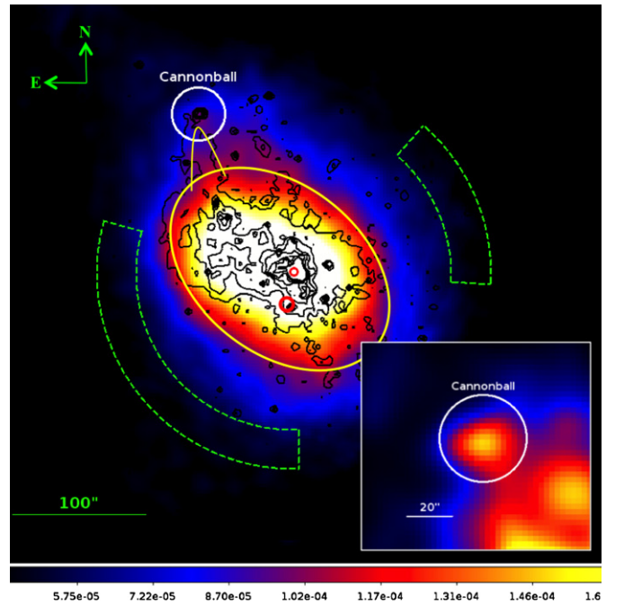
Figure 1. NuSTAR mosaic image of the Cannonball, Plume, and Sgr A* region in 3–79 keV band. The Cannonball is indicated by the white circle with radius of 20'' . Background regions are indicated by the green dashed regions. Chandra 3–8 keV contours are overlaid in black, and approximate positions of the Plume and Sgr A East are in yellow. The image is shown with a linear color scale and the scale range chosen to highlight the Cannonball emission. Inset: NuSTAR mosaic image of the Cannonball in 10–30 keV band.
