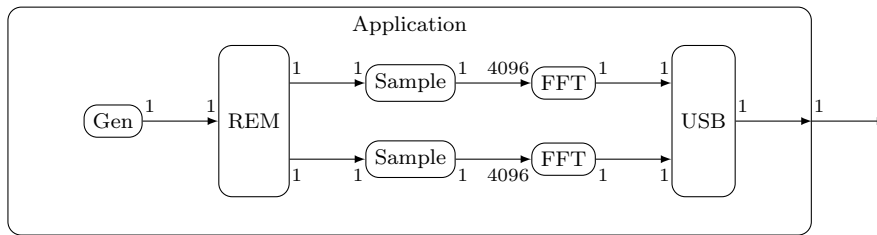
Figure 4: Simplified behavioural model of the product. This is a setup where two channels are actively being used.
