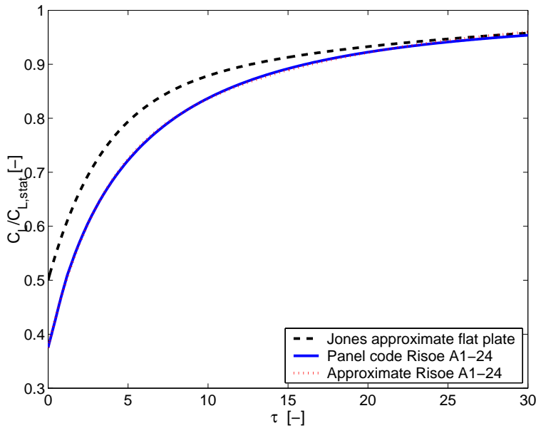
Figure 11. Inviscid response of the lift to a step change in angle of attack for a flat plate and a Risø A1-24 airfoil. \tau = 2U_0t/c
