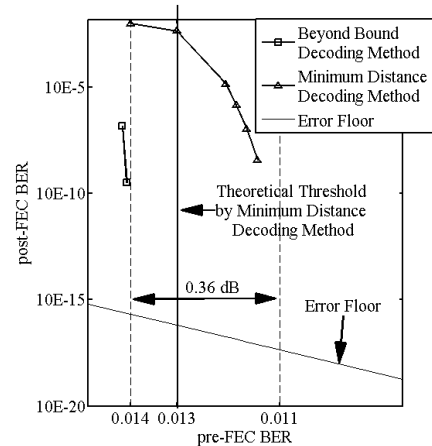
Fig. 2 Simulation Result
