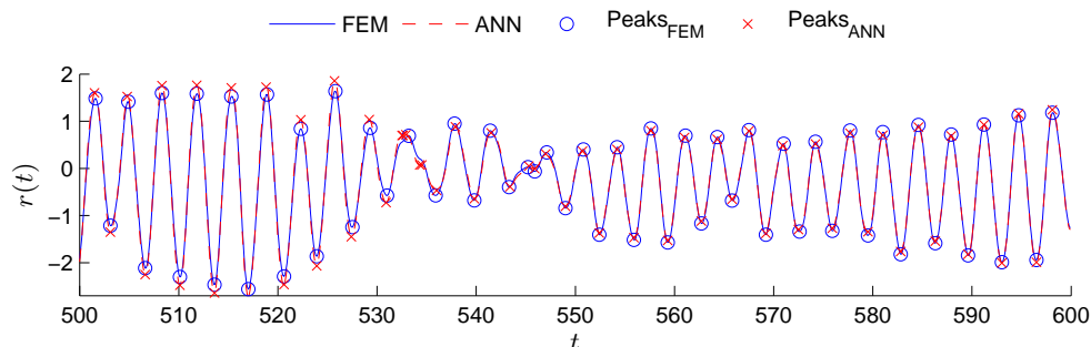
Figure 4. Exact FEM solution together with ANN simulation.
