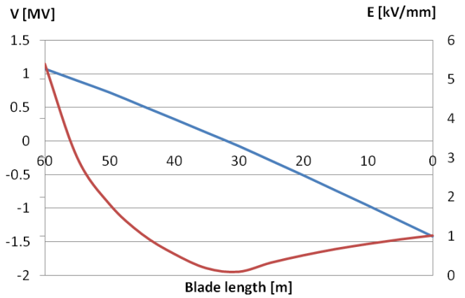
Fig. 16. Maximum voltage difference V [MV] between the lightning conductor and the wire (blue trace) and average electric field E [kV/mm] (red trace) for case 2. Current impulse corresponding to the first return stroke positive.
