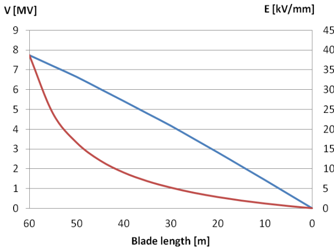
Fig. 14. Maximum voltage difference V [MV] between the lightning conductor and the wire (blue trace) and average electric field E [kV/mm] (red trace) for case 1. Current impulse corresponding to the first return stroke negative.
