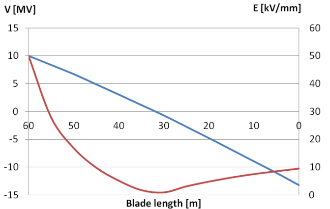
Fig. 18. Maximum voltage difference V [MV] between the lightning conductor and the wire (blue trace) and average electric field E [kV/mm] (red trace) for case 2. Current impulse corresponding to the subsequent return stroke.
