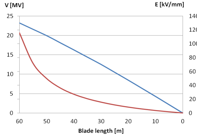
Fig. 15. Maximum voltage difference V [MV] between the lightning conductor and the wire (blue trace) and average electric field E [kV/mm] (red trace) for case 1. Current impulse corresponding to the subsequent return stroke.
