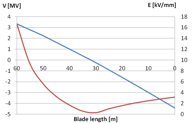
Fig. 17. Maximum voltage difference V [MV] between the lightning conductor and the wire (blue trace) and average electric field E [kV/mm] (red trace) for case 2. Current impulse corresponding to the first return stroke negative.
