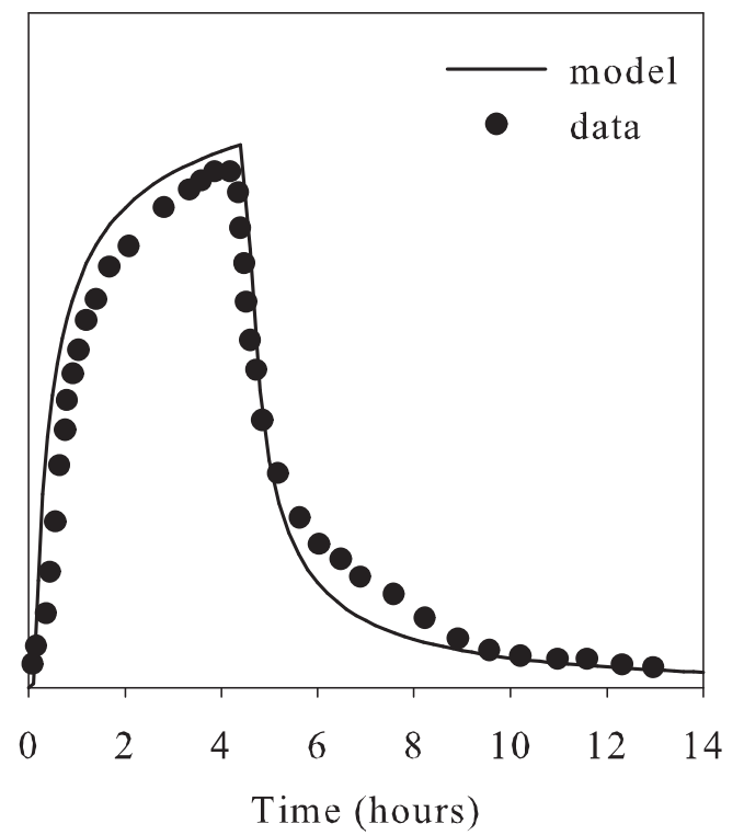
Chloride
