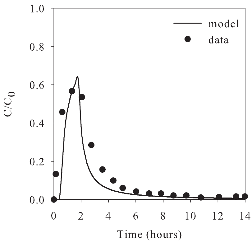
MCPP
