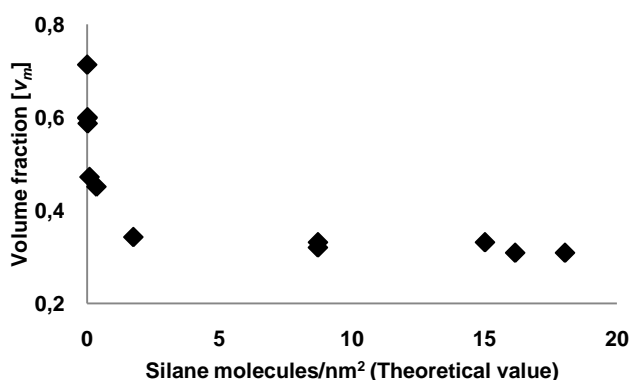
Fig. 3 Volume fraction of monoclinic zirconia in MPTMS modified samples in ambient atmosphere as a function of the theoretical number of silane molecules per \text{nm}^2
