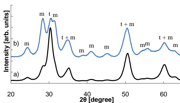
Fig. 2 XRD patterns for zirconia silanized with MPTMS exposed to air (a) and unmodified zirconia exposed to air (b) t=tetragonal reflection, m=monoclinic reflection.
