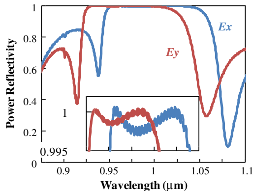
Fig. 4. (Color online) Calculated power reflectivity spectra (for E_x and E_y linear polarizations) of the optimized HCG with an asymmetric fabrication error, W_x = 183 nm, W_y = 173 nm.
