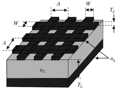
Fig. 1. Polarization-independent HCG with a single layer of cross stripes for simple fabrication.
