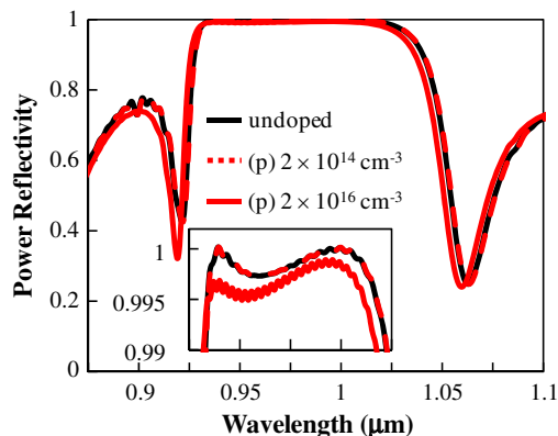
Fig. 5. (Color online) Calculated power reflectivity spectra of the optimized HCG with the absorption coefficients of 0.4 and 29.3 \text{cm}^{-1} at the doping levels of (p) 2 \times 10^{14} \text{cm}^{-3} and (p) 2 \times 10^{16} \text{cm}^{-3} , respectively.
