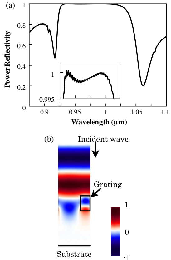
Fig. 2. (Color online) (a) Calculated power reflectivity spectrum of the optimized HCG ( \Lambda = 556 nm, W = 178 nm, T_g = 270 nm, T_L = 630 nm, n_g = 3.5 , n_L = 1 ). (b) The electric field distribution (linear polarization perpendicular to the paper) in the unit cell for a wavelength within the high-reflectivity band.
