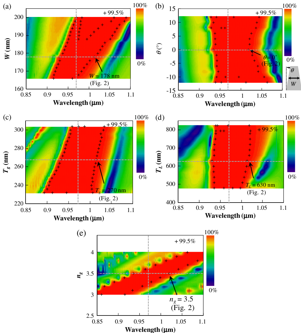
Fig. 3. (Color online) (a) W , (b) \theta , (c) T_g , (d) T_L , and (e) n_g dependences of the reflectivity spectrum. The other parameters are the same as those in Fig. 2. The symbol “+” indicates 99.5%.
