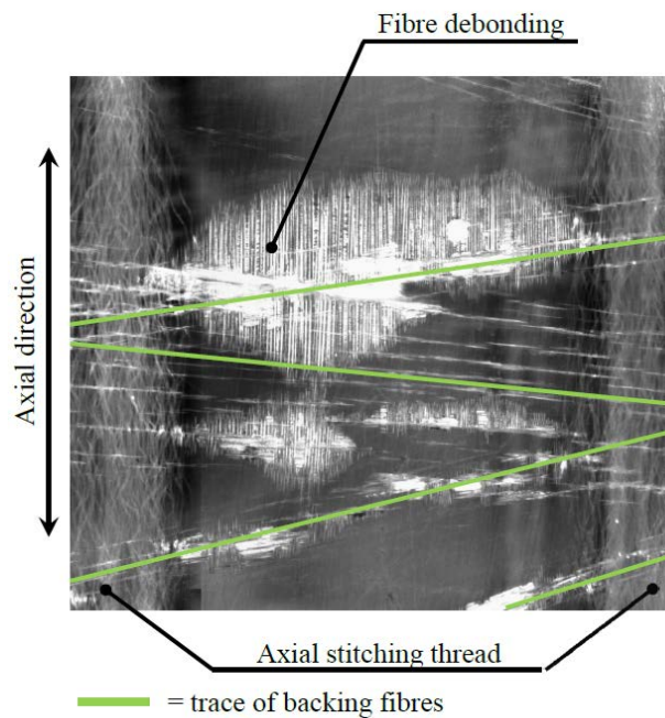
Figure 5. Magnification of the red box in Fig. 4 showing fibre debonding in the axial fibres beneath the backing layer.
