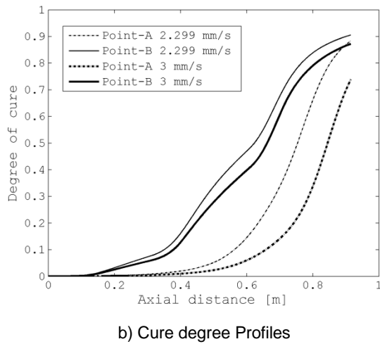
Figure 8. Temperature (a) and cure degree (b) profiles at points A and B for Case-1.
