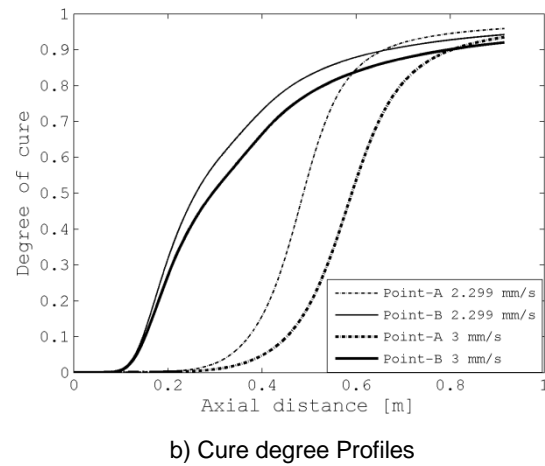
Figure 9. Temperature (a) and cure degree (b) profiles at points A and B for Case-2.
