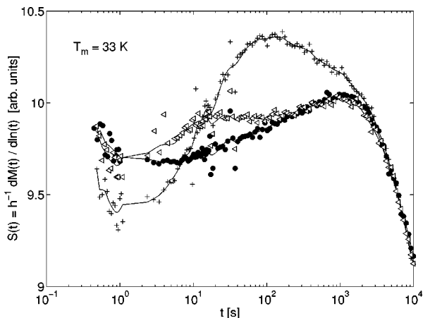
FIG. 9. Relaxation rate S(t) vs time. The sample has been aged for 1 h 30 min at T_m = 33 K and afterward subjected to a negative temperature cycling \Delta T during t_{w_2} . Circles: \Delta T = 0 ; plus signs: T_m + \Delta T = 28 K, t_{w_2} = 7 h; triangles: T_m + \Delta T = 23 K, t_{w_2} = 10 h. H = 0.05 Oe.
