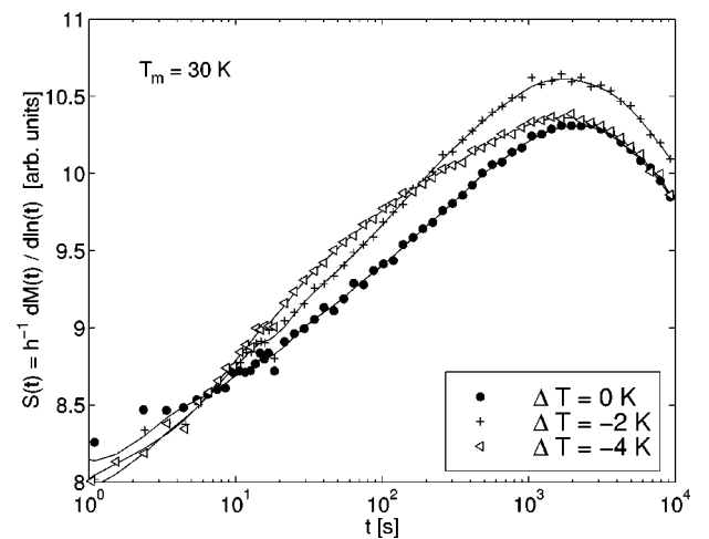
FIG. 4. Relaxation rate S(t) vs time. The sample has been aged t_{w_1} = 3000 s at T_m = 30 K and afterward subjected to a negative temperature cycling \Delta T during t_{w_2} = 10\,000 s, immediately prior to the application of the field H = 0.05 Oe; circles: \Delta T = 0 , t_{w_2} = 0 ; plus signs \Delta T = -2 K; triangles: \Delta T = -4 K.
