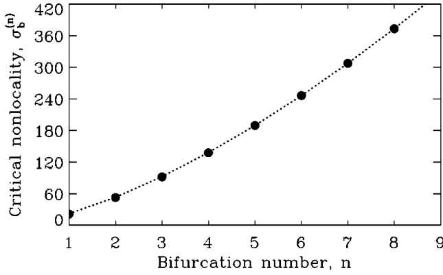
FIG. 2. Focusing nonlocal medium with 4s\rho_0=1 and rectangular response function. Bifurcation values of the nonlocality parameter \sigma_b^{(n)} (dots) versus bifurcation number n . The dashed line shows approximation (52).
