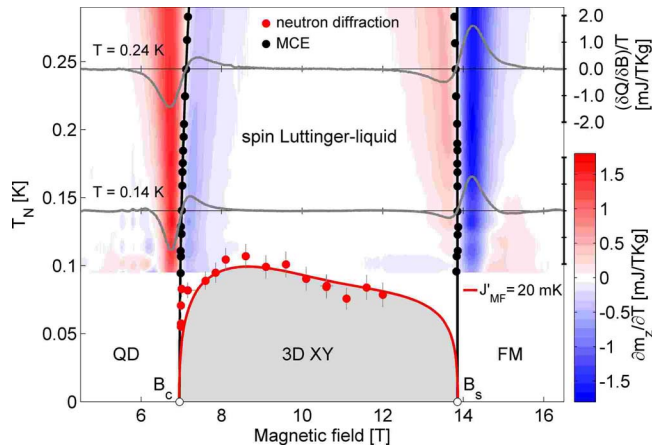
FIG. 1. (Color online) Low- T phase diagram of (\text{Hpip})_2\text{CuBr}_4 . The crossover temperature to the spin-LL phase is derived from MCE measurements and the phase transition to the BEC (3D-XY magnetic order) from neutron diffraction. The contour plot is based on 18 individual field scans of the MCE (two shown as gray lines), using (\partial Q/\partial B)/T = -(\partial m_z/\partial T)|_B (Ref. 15). The red line is based on a theoretical fit (see text).
