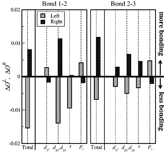
FIG. 3. The change in left and right partial OP, \{O_{12}^L, O_{12}^R\} and \{O_{23}^L, O_{23}^R\} for a change in bias from 0 to 1 V for the (100) wire. These are broken into main orbital contributions with respect to the middle atom (2). We show the sum of the contributions for the degenerate d_{yz} and d_{zx} .
