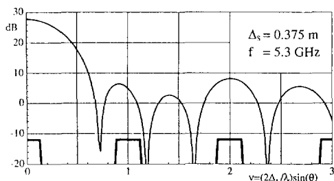
Fig. 6: Azimuth pattern for minimum ambiguity; Processed band and aliasing bands for resolution 1.5 m.
