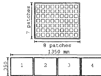
Fig. 3: Microstrip antenna for 5.3 GHz SAR
