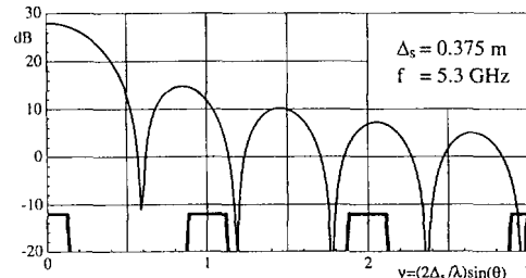
Fig. 4: Processed band and aliasing bands; resolution 1.5 m.
