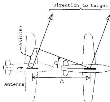
Fig. 1: SAR geometry in the horizontal plane
