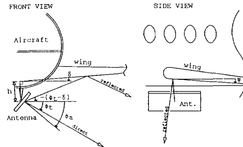
Fig. 8: Antenna and wing reflection geometry.
