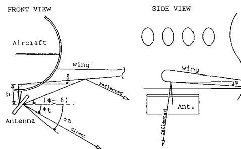
Fig. 8: Antenna and wing reflection geometry.
