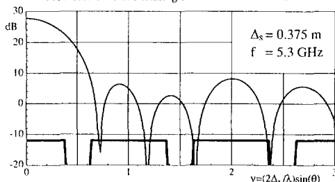
Fig. 7: Azimuth pattern for minimum ambiguity; Processed band and aliasing bands for resolution 0.5 m.
