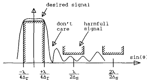
Fig. 2: Outline of azimuth radiation pattern
