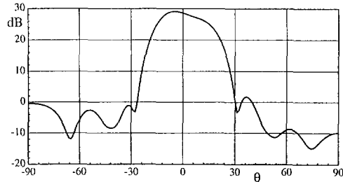
Fig. 9: Antenna pattern in elevation
