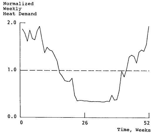
Figure 1. The Week Averaged Heat Demand through the Year.
