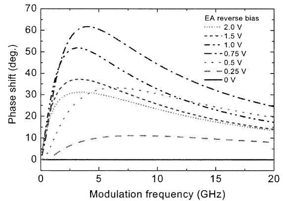
Fig. 6. Calculated phase shift (relative to an EA bias of 0 V) for different values of the bias voltage to the two EAs. The input power was 5.3 dBm.
