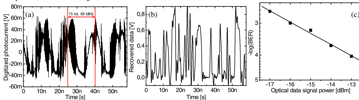
Fig. 4 (a) Time trace of digitized photocurrent. (b) Recovered 1.25 Gb/s data using the DSP based receiver from Figure 1. (c) BER as a function of optical data signal power.
