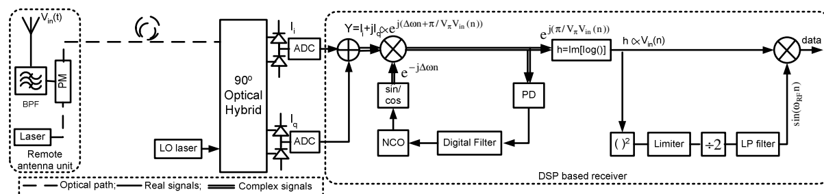
Fig. 1 General outline of a DSP based coherent receiver for RoF links. PM: optical phase modulator, BPF: band-pass filter. NCO: number controlled oscillator, PD: phase detector, \Delta\omega : frequency difference between transmitter and LO laser and \Delta\omega = 2\pi\Delta f .
